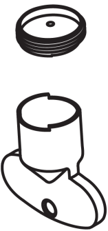
99823579 AERATOR KIT
